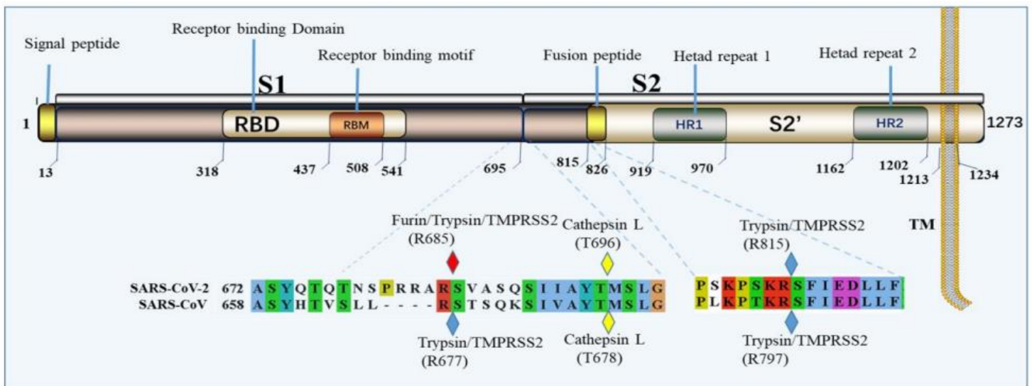
Figure 2. Sequence analysis of Spike protein in SARS-CoV-2. It contains an N-terminal signal peptide, S1 and S2. S1 contains
